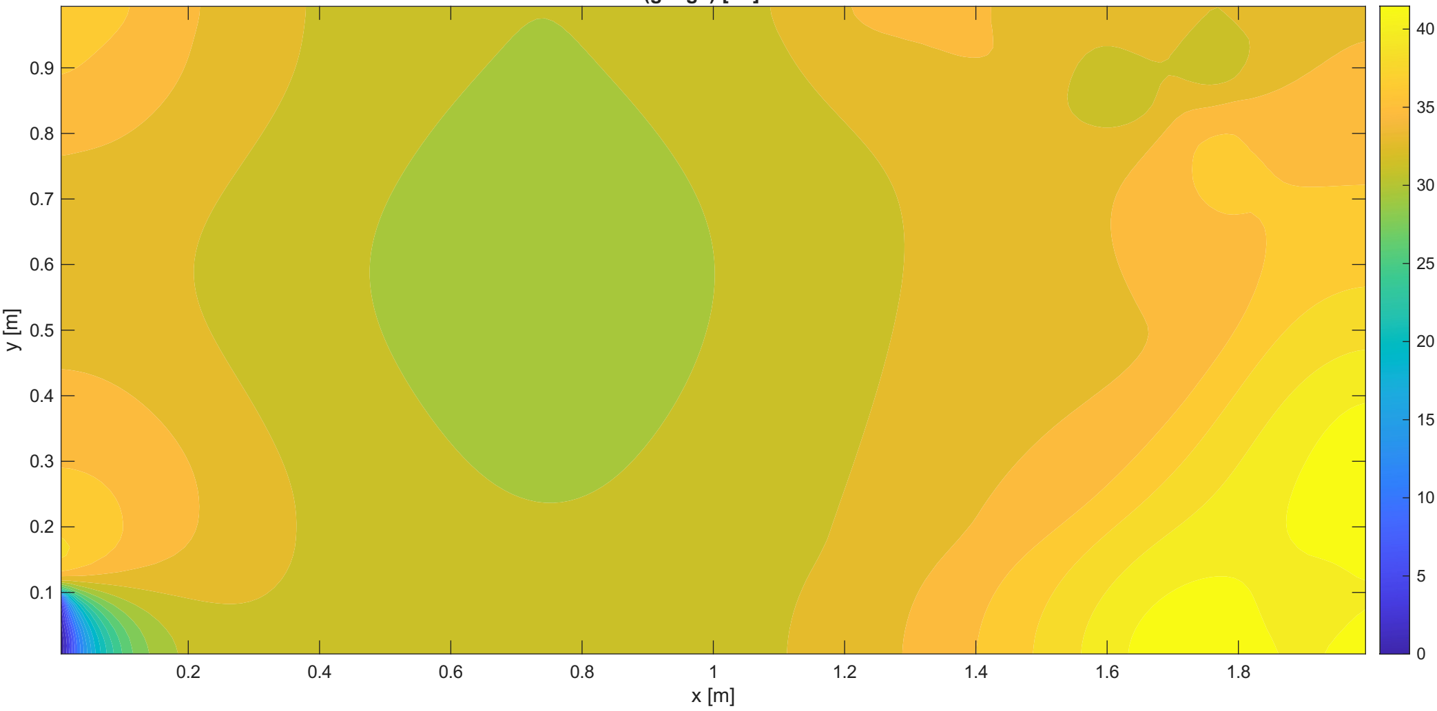
Pressure (gauge) [Pa] — 160×80
